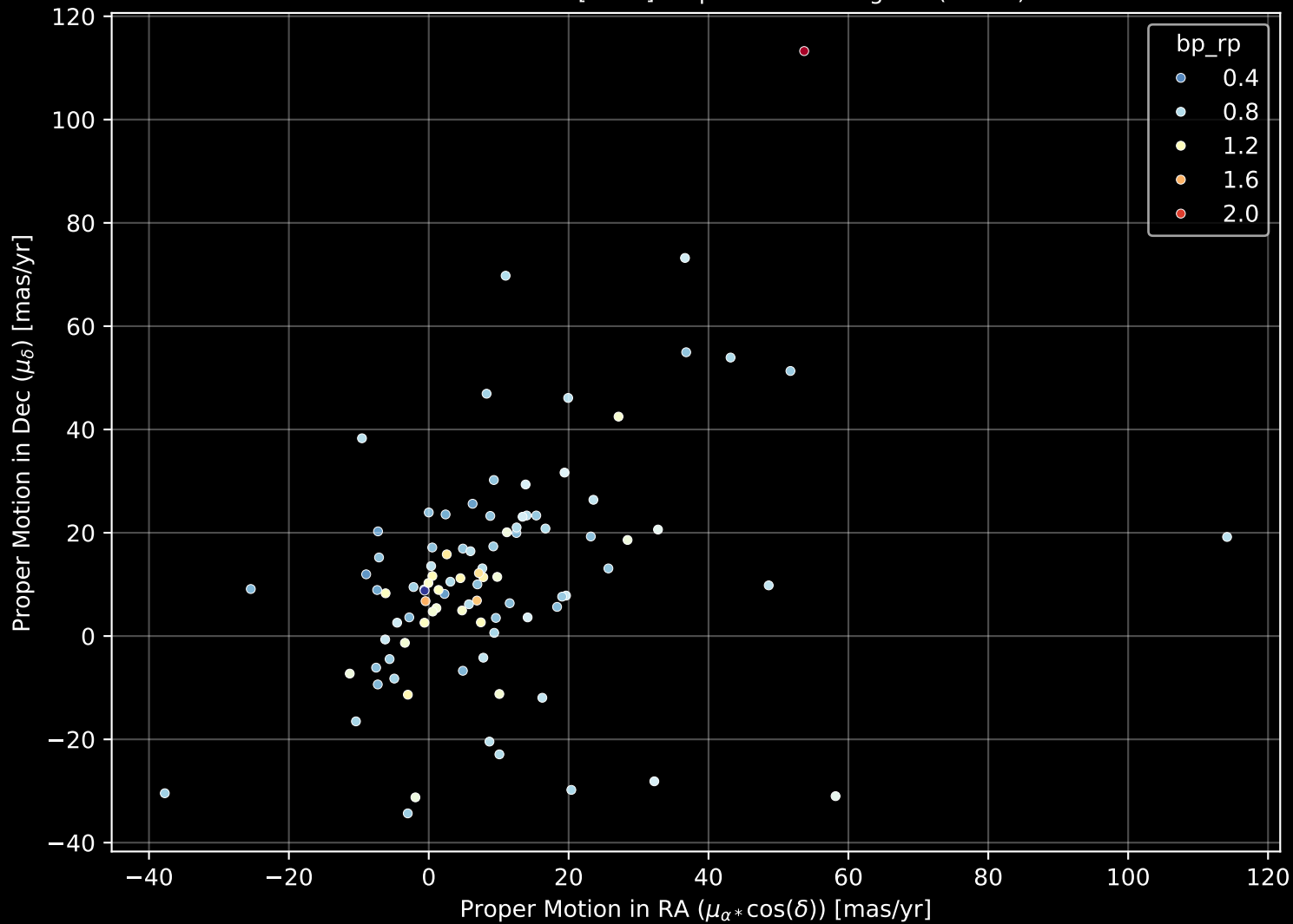
GALAH DR4 Field: [7181] Proper Motion Diagram (n= 95)
