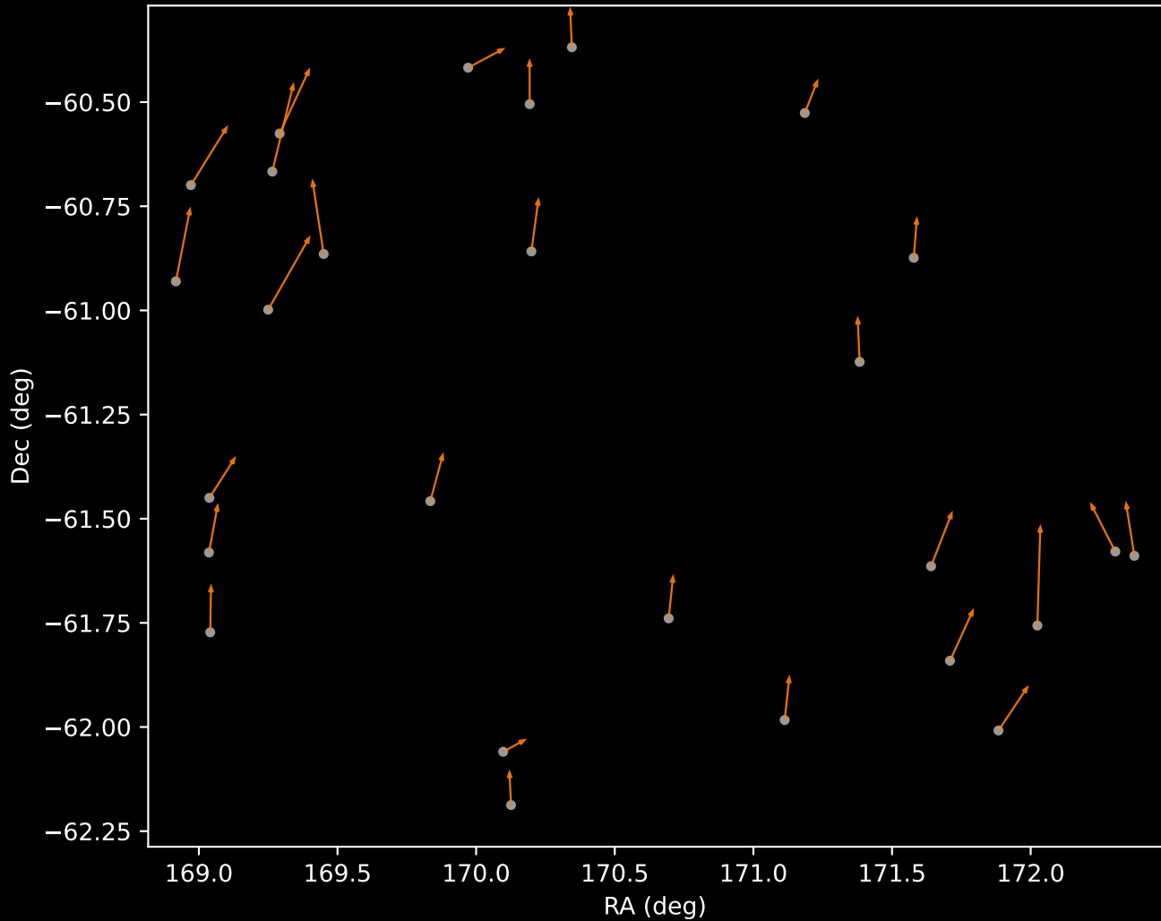
GALAH DR4 Cluster 2 Proper Motion Vectors (n=27)
