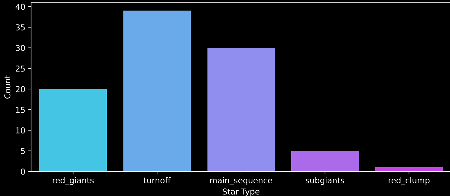
GALAH DR4 Field: [7181] Count plot of Star Type
