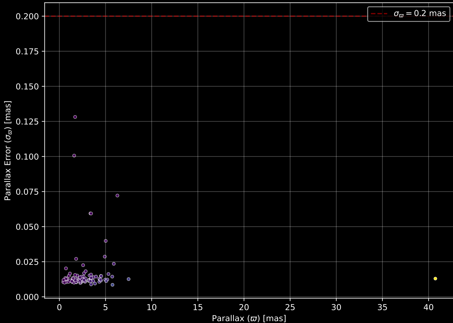
GALAH DR4 Field: [7181] Parallax Quality (n= 95)
