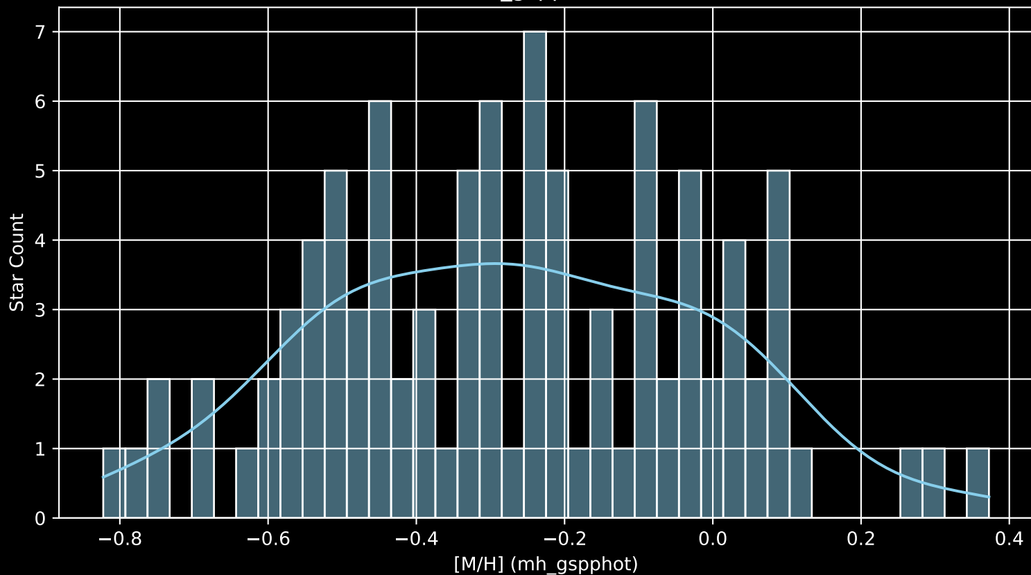
GALAH DR4 Field: [7181] [M/H] (mh_gspphot) (n= 95)
