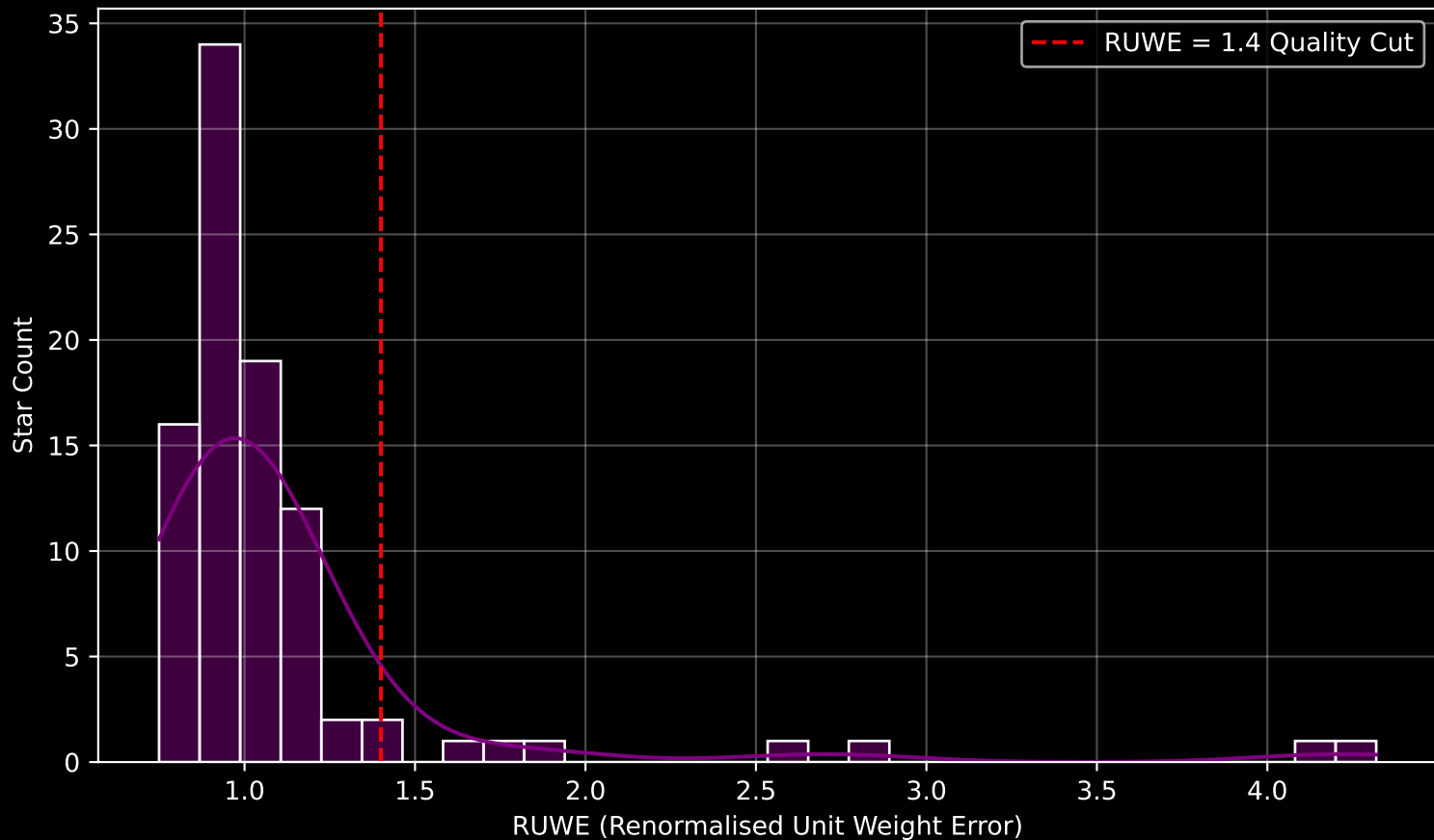
GALAH DR4 Field [7181] RUWE Distribution (n= 92)
